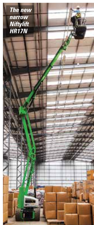
Mast booms have a useful up and over capability
